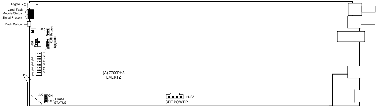
Figure 7-1: 7760CCM-HD Jumpers
