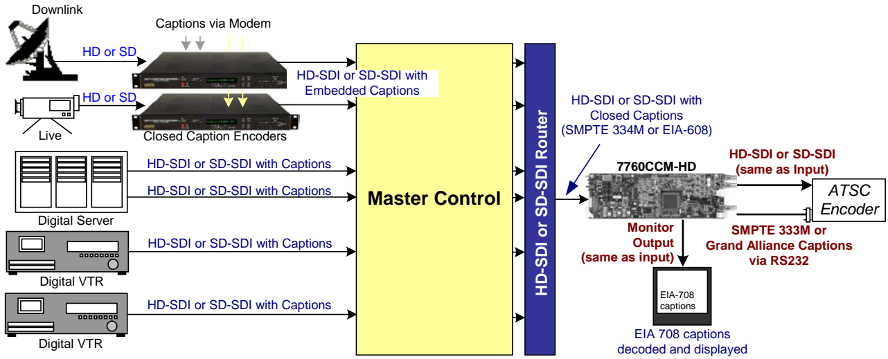
Figure 1-2: 7760CCM-HD Application Diagram
