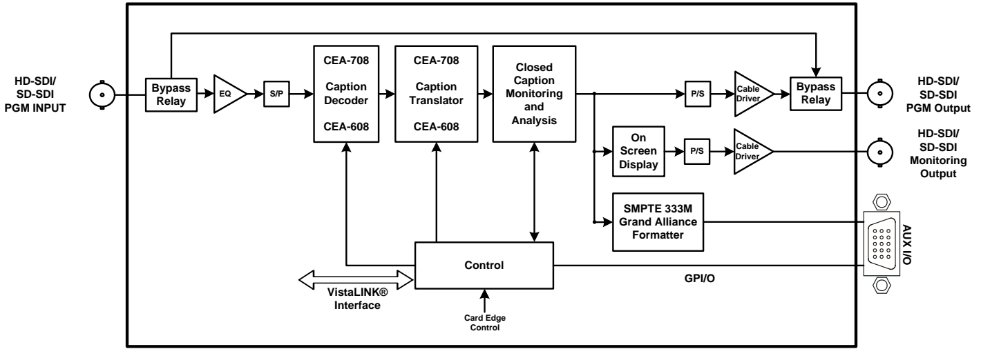
Figure 1-1: 7760CCM-HD Block Diagram
