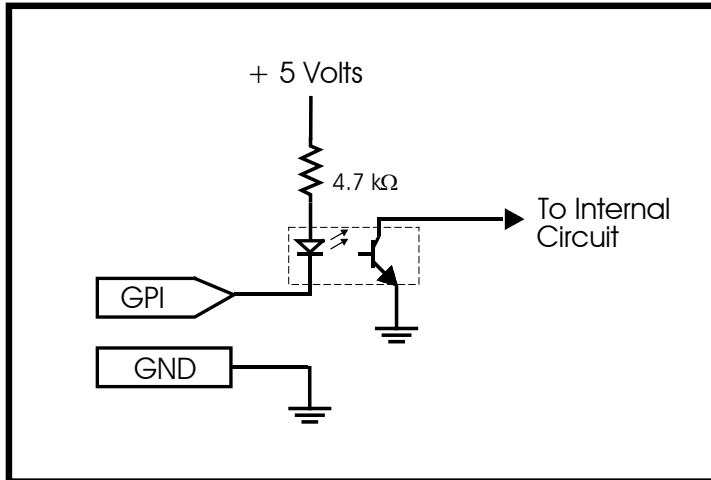
Figure 2-2: GPI Input Circuitry
