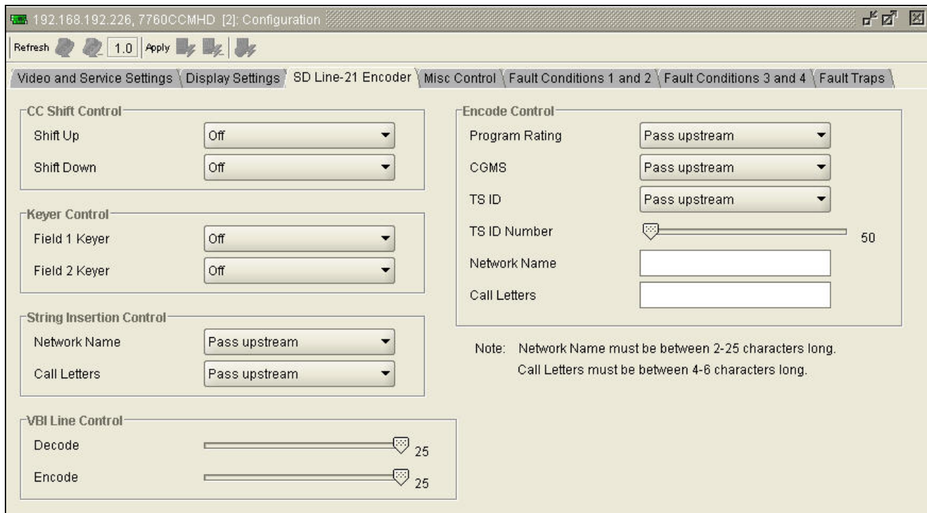
Figure 9-3: SD Line-21 Encoder Window
