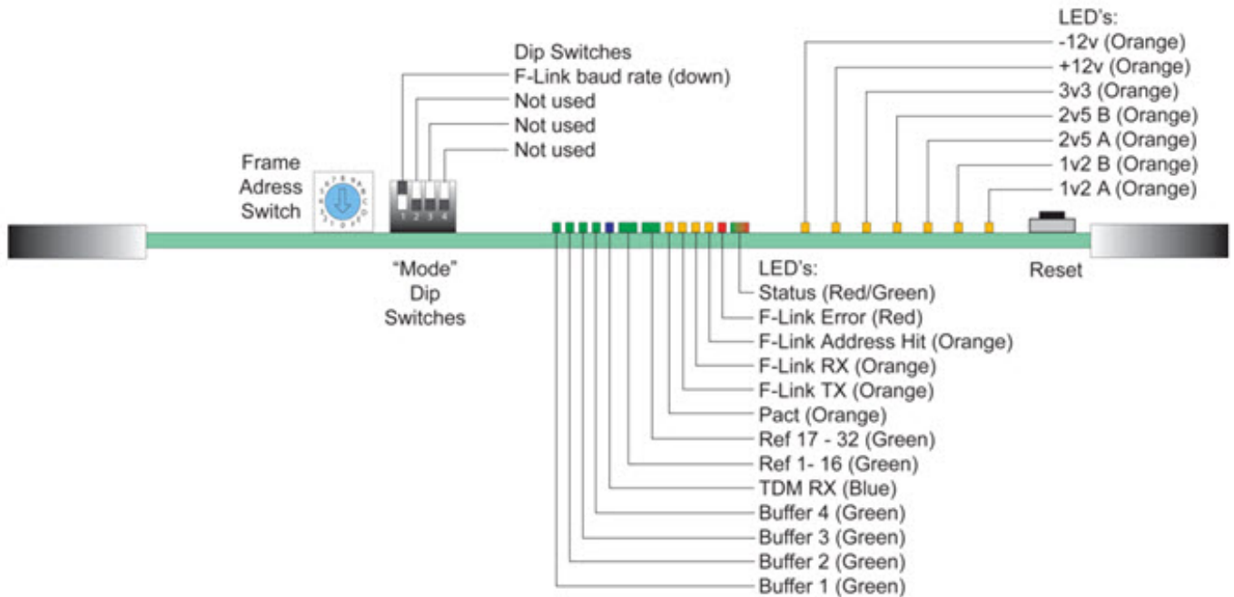
Figure 5-21: AES Digital Audio Input Card (Viewed from the Front)
