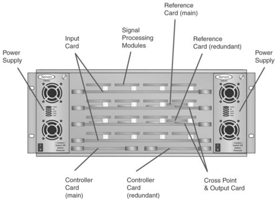
Figure 5-2: 64x64 Digital Video Xenon – Front View
