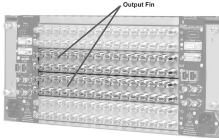
Figure 5-24: Digital Video BNC Connector Output Fins Mounted in the Xenon Frame
