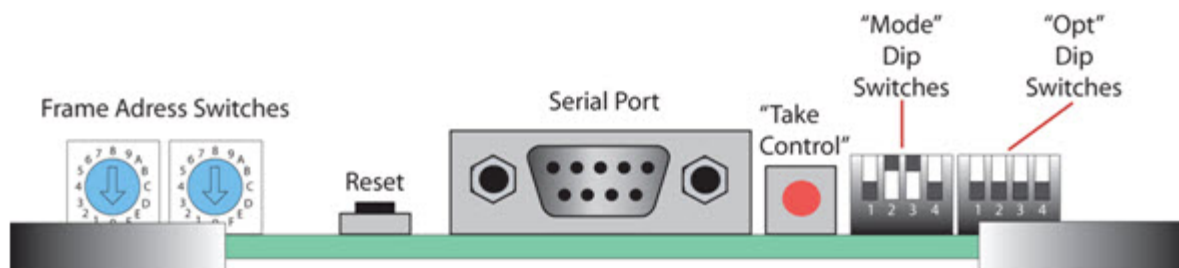
Figure 5-60: Control Module Switches (Viewed from the Front)
