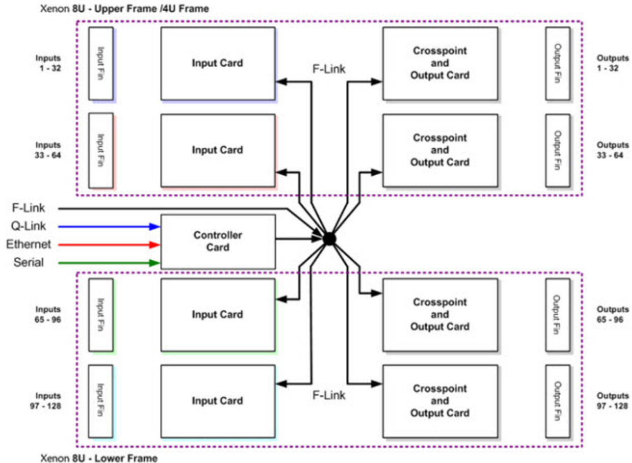
Figure 5-58: Control Module – Block Diagram
