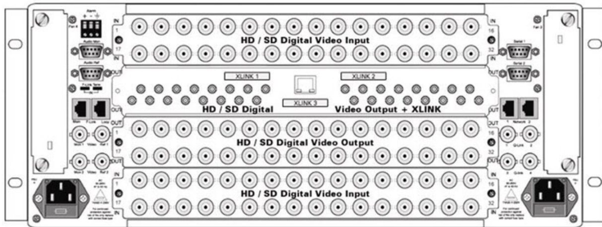
Figure 5-29: 4RU Xenon with One X-LINK® Output Card Installed
