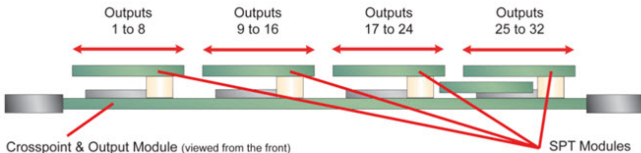
Figure 5-54: SPT Location (Old Crosspoint & Output Module)
