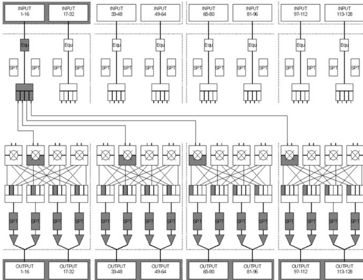
Figure 9-2: One to All Mapping
