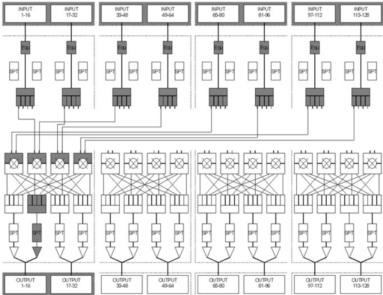
Figure 9-3: All to One Mapping
