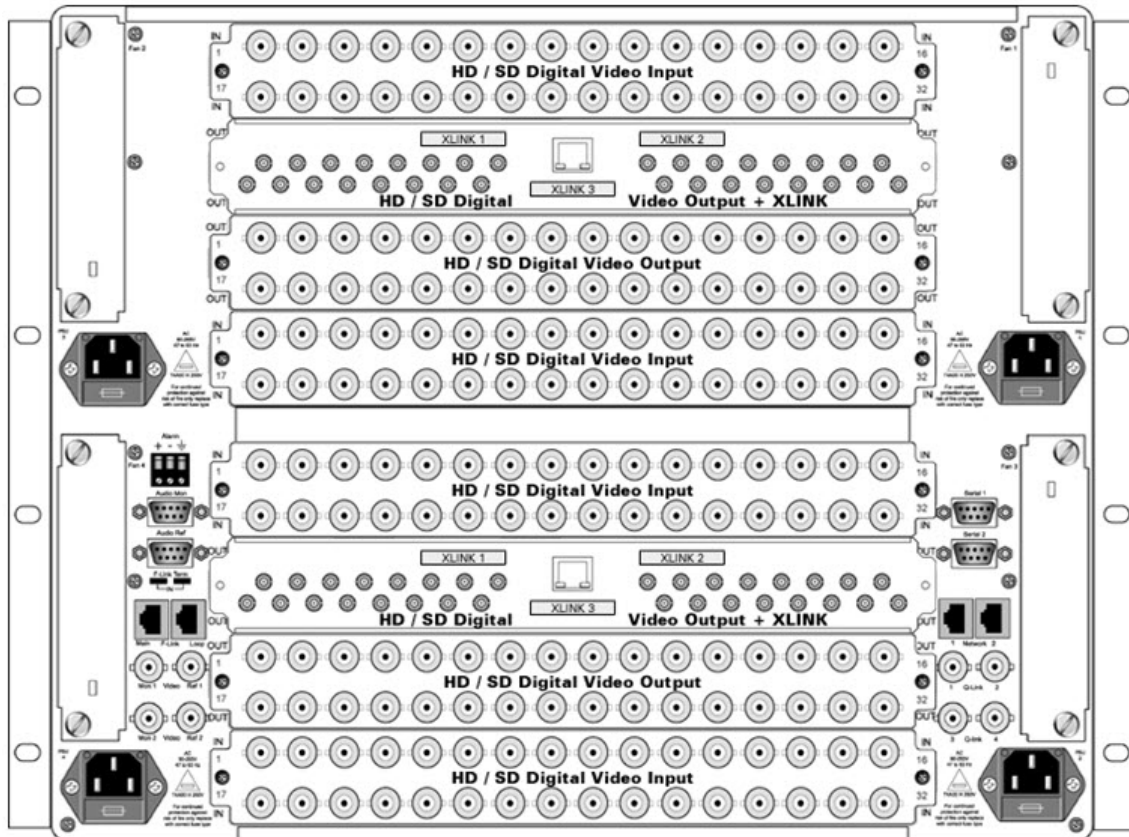
Figure 5-30: 8RU Xenon with Two X-LINK® Output Cards Installed
