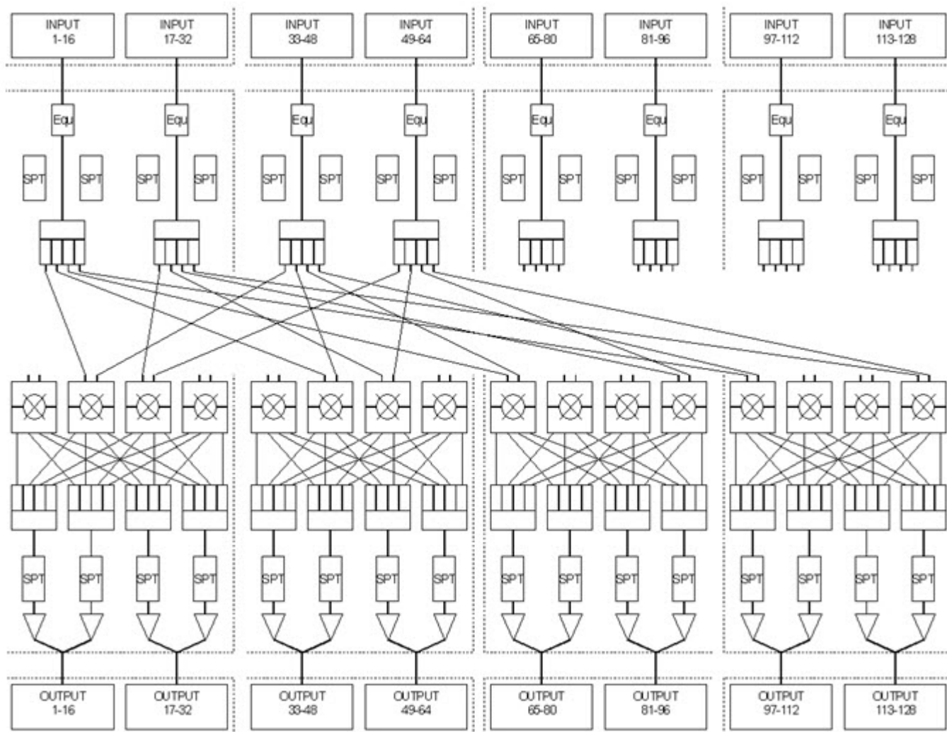
Figure 9-1: Xenon Signal Path
