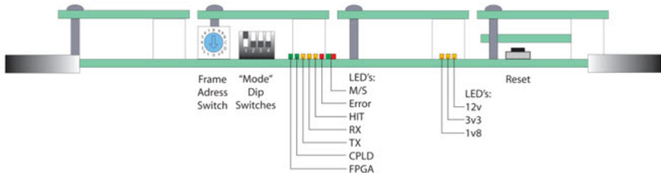
Figure 5-38: Crosspoint & Output Card Switches & LED's (Viewed from the Front)
