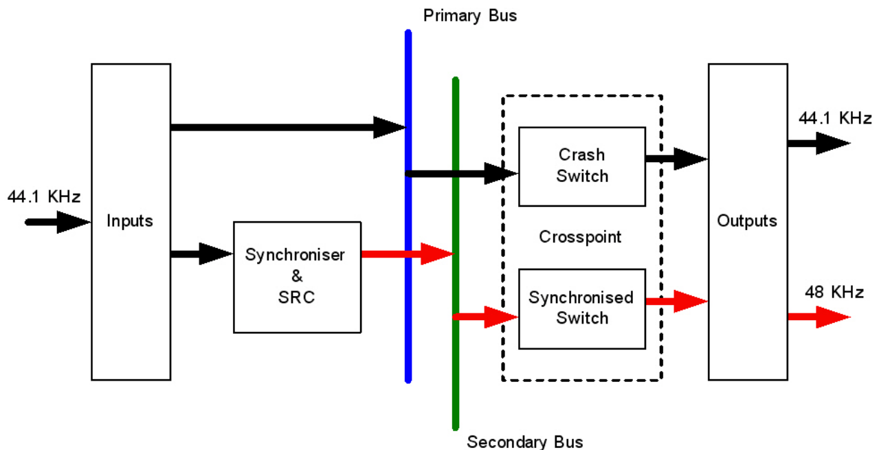
Figure 5-20: Xenon Router Dual Path Routing
