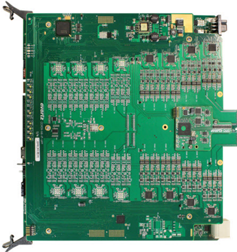
Figure 5-22: Analog Audio Input Card
