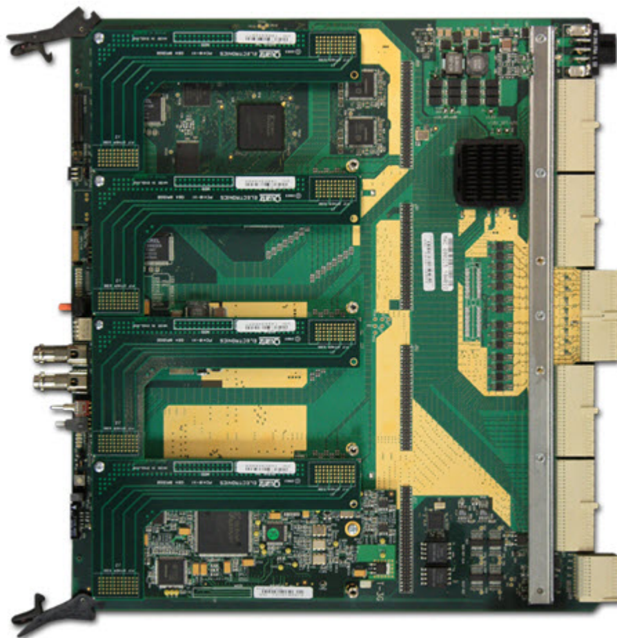
Figure 5-37: Crosspoint & Output Card
