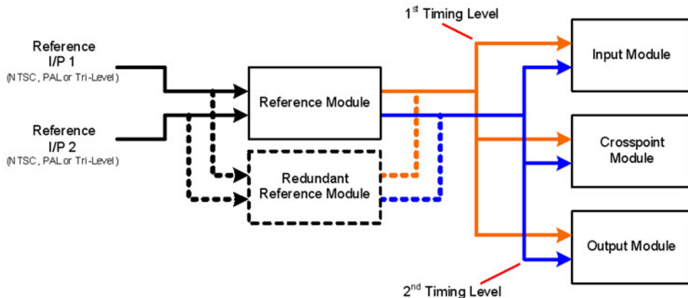
Figure 5-63: Generation of Independent Timing Levels
