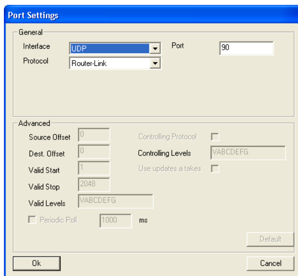
Figure 8-9: Ethernet Panels Port Settings
