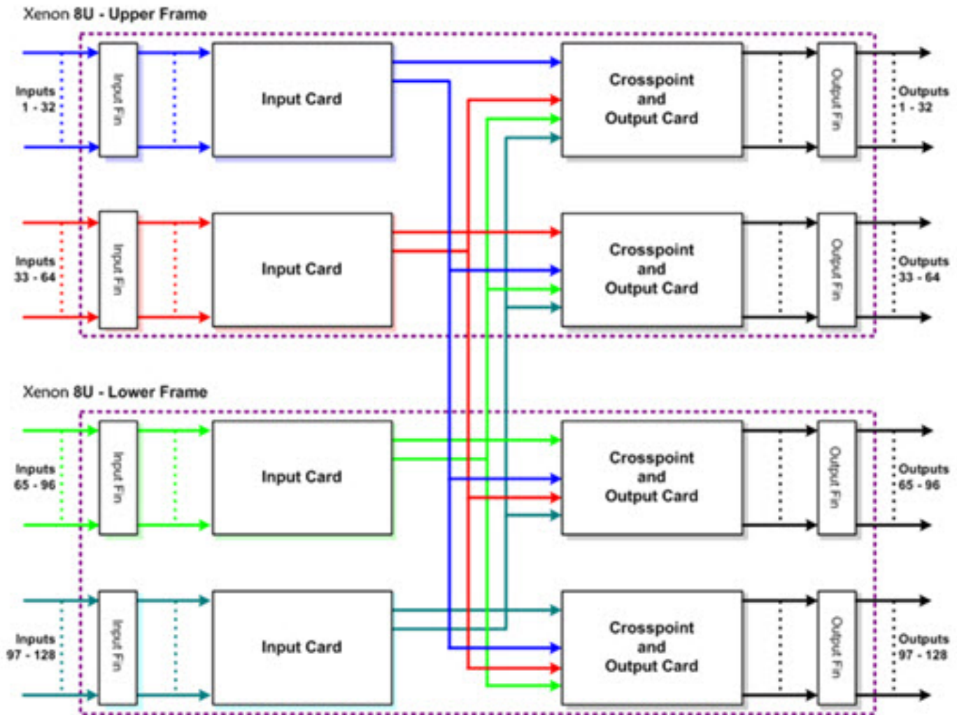
Figure 5-4: 8RU Xenon Block Diagram
