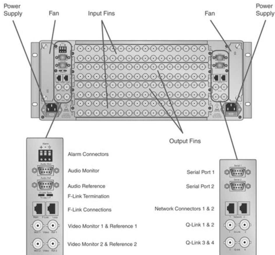
Figure 5-3: 64x64 Digital Video Xenon – Rear View
