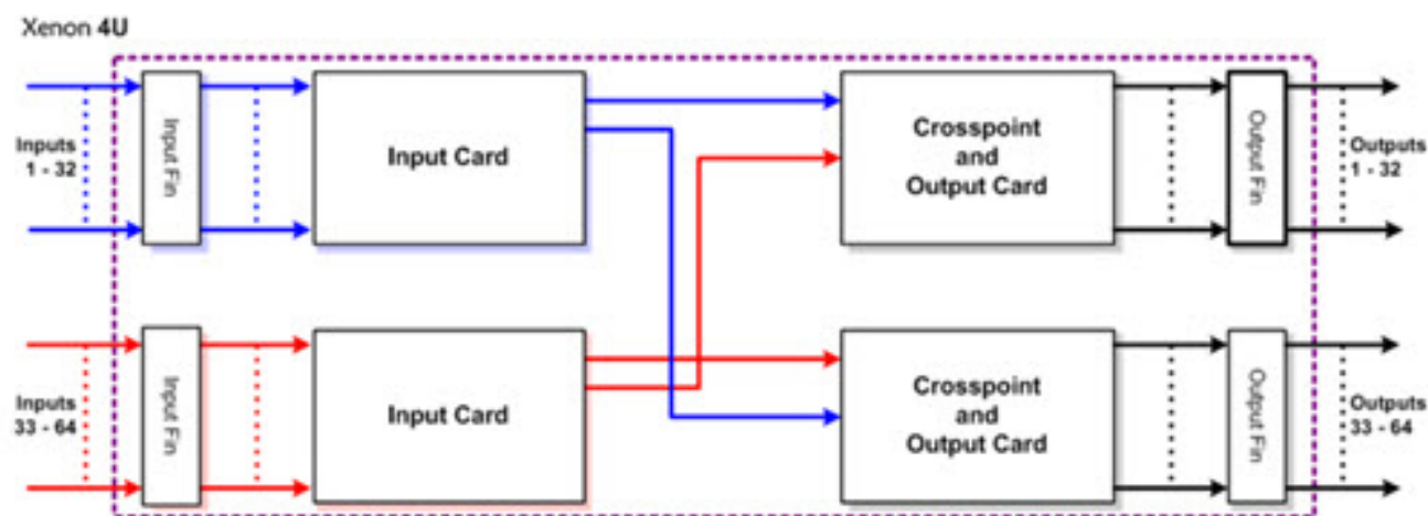
Figure 5-1: 4RU Xenon Block Diagram
