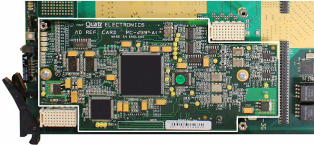
Figure 5-62: Reference Module Mounted on the Crosspoint & Output Card
