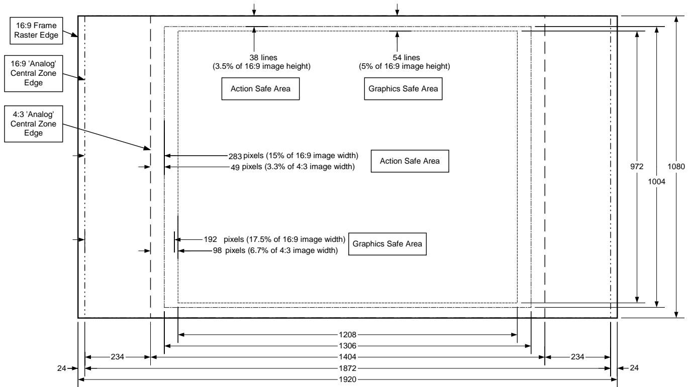
Figure 8-2: Australian 16:9 Shoot and Protect 4:3 Safe Areas for SD Analog Transmission
