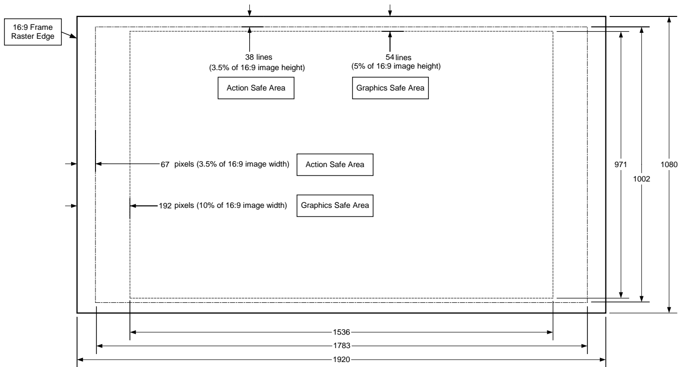
Figure 8-1: Australian 1080i 16:9 HD transmission Safe Areas
