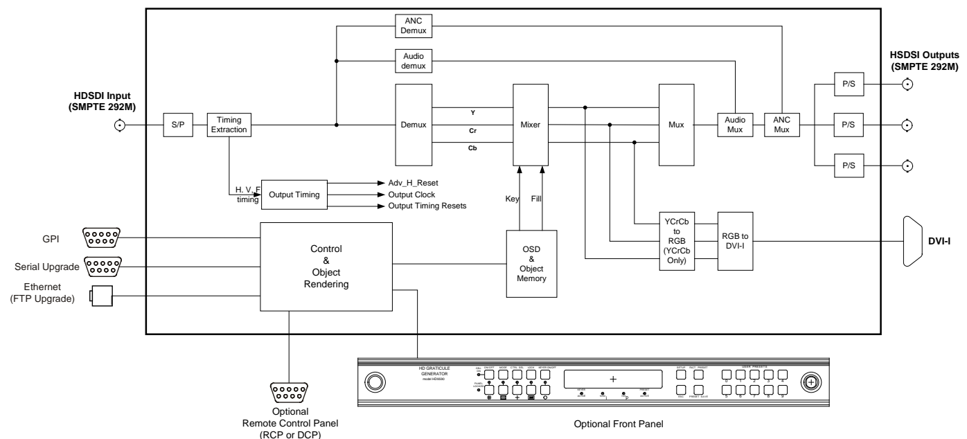
Figure 1-1: HD9690 Block Diagram
