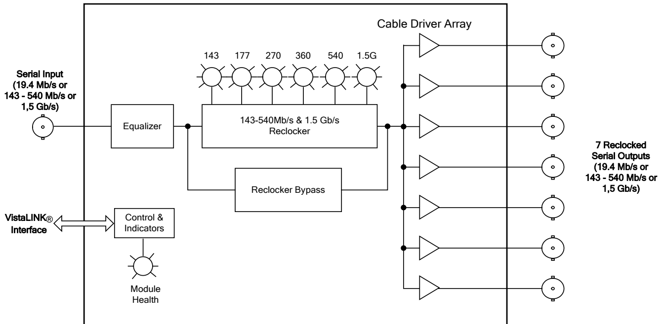
Figure 1-1: 7700DA7-HD Block Diagram
