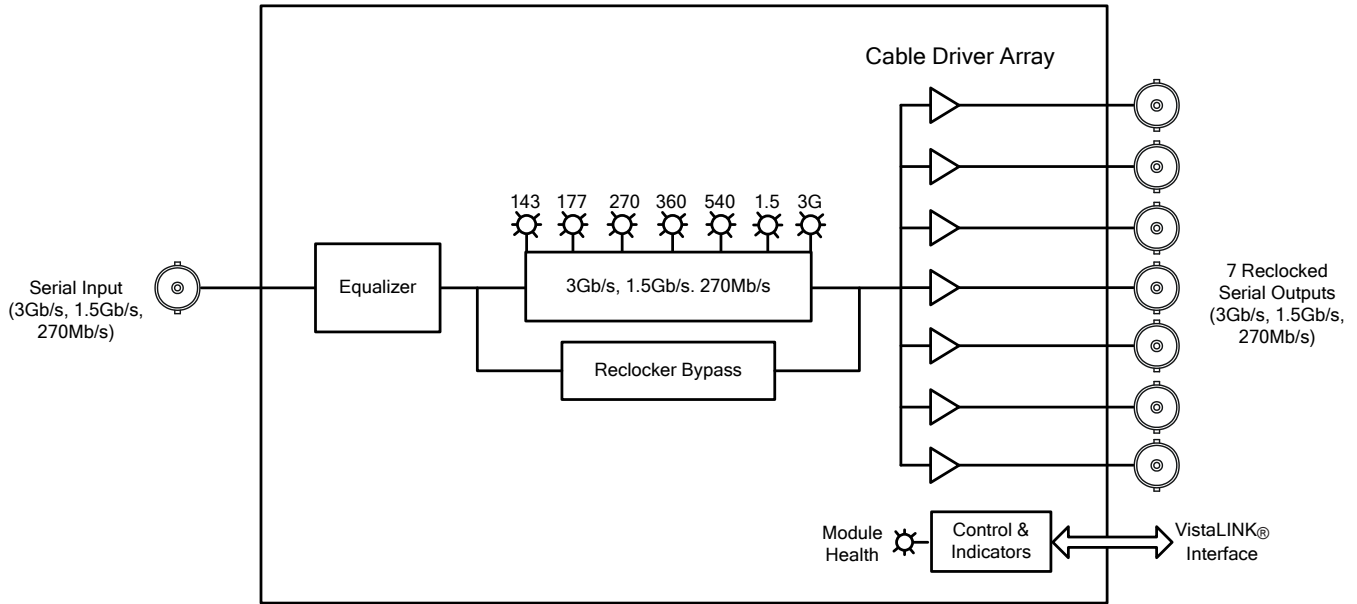
Figure 1-1: 7700DA7-3G Block Diagram
