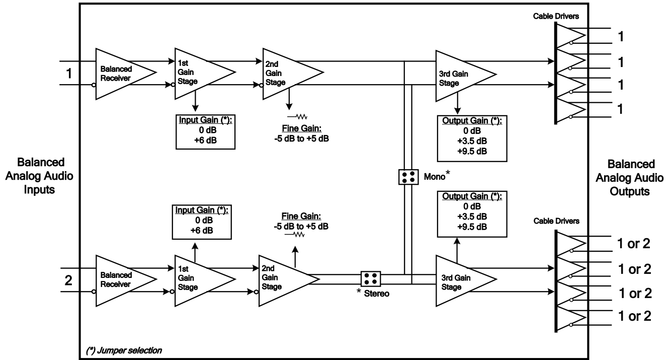
Figure 1-2: 7700ADA-AUD Block Diagram Rev A
