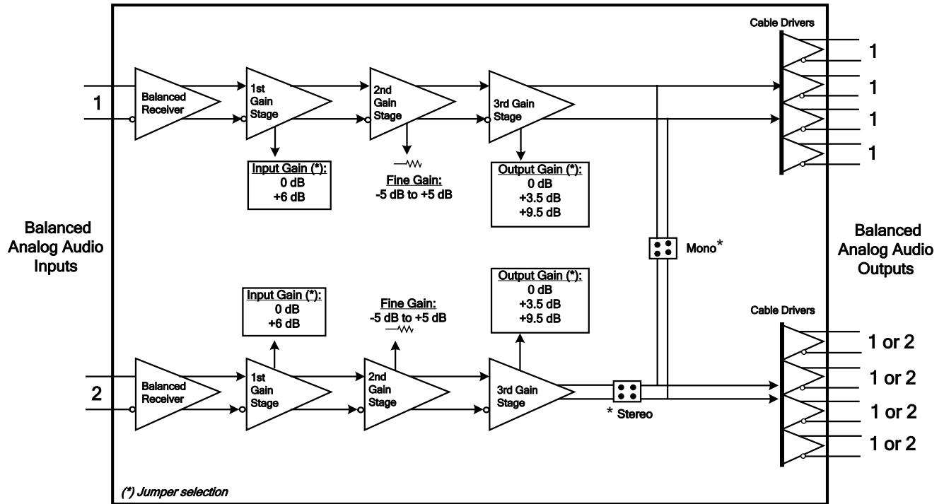
Figure 1-3: 7700ADA-AUD Block Diagram Rev B
