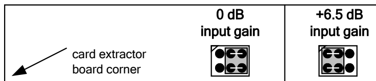
Figure 6-7: Setting the Input Gain Level on PCB Rev 2
