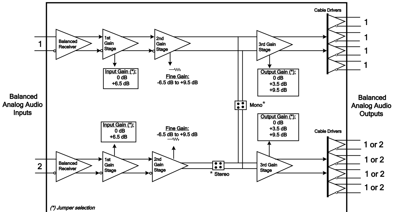
Figure 1-1: 7700ADA-AUD Block Diagram Rev 2
