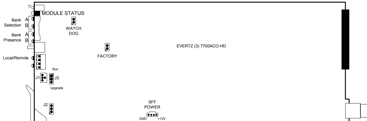
Figure 7-1: Location of Jumpers – Rev 3 Main Board
