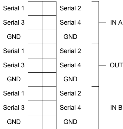
Figure 2-2: Control Connection Pin Out
