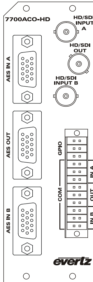
Figure 2-1: Rear Panel
