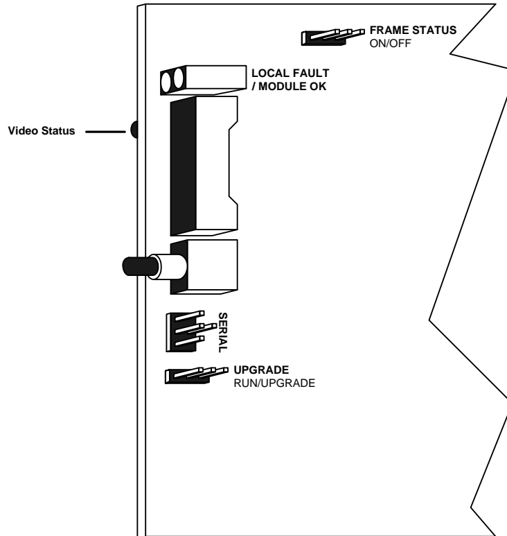
Figure 4-1: 7707OE-3G-1 Status Indicator and Jumper Locations
