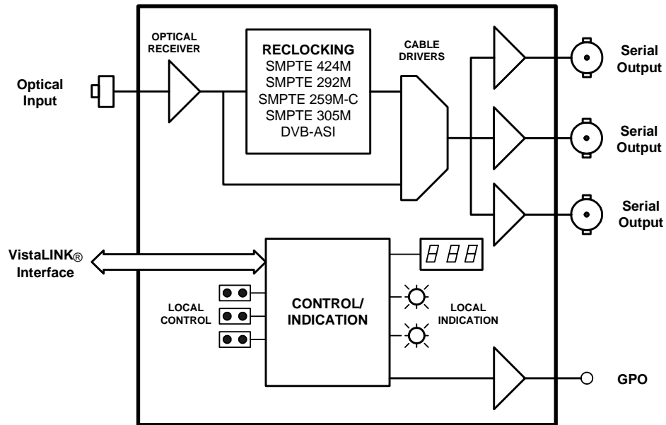
Figure 1-1: 7707OE-3G-1 Block Diagram
