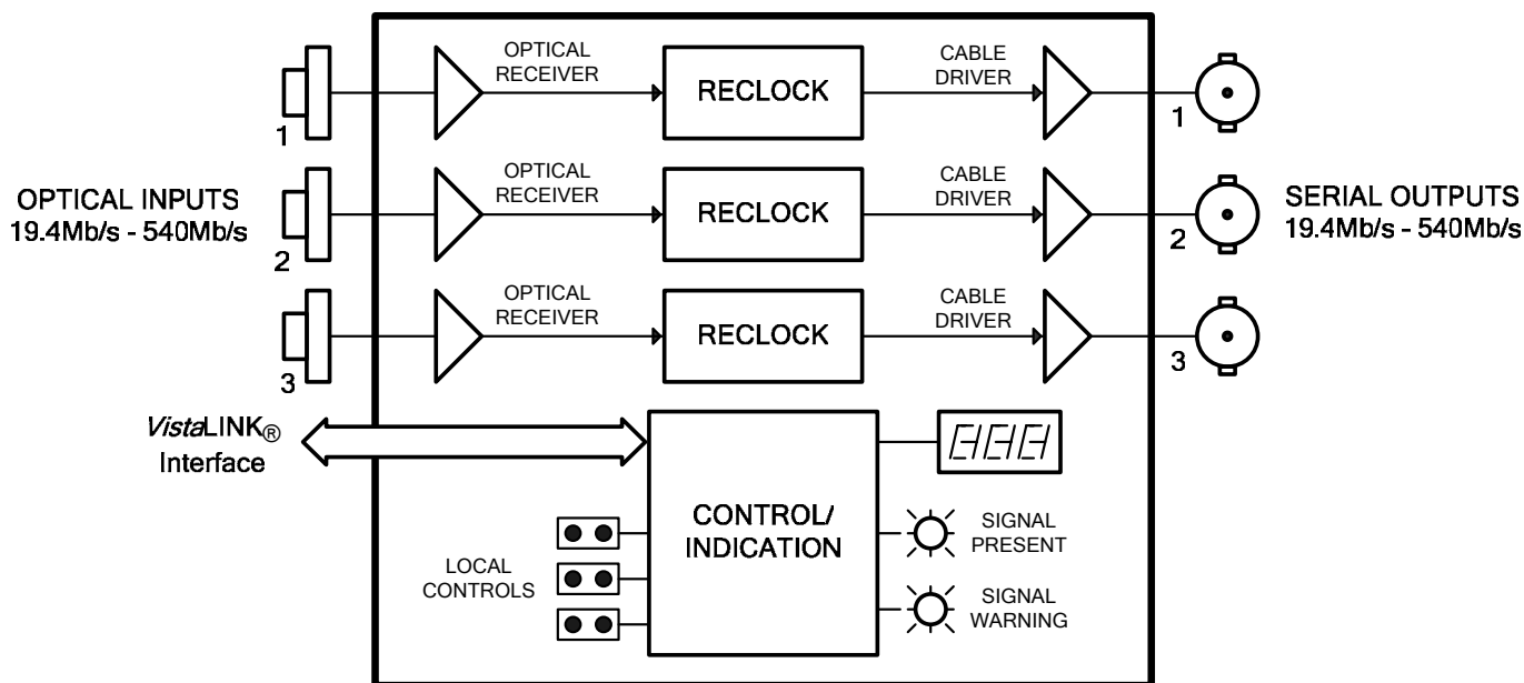
Figure 1-1: 7707OE-3 Block Diagram
