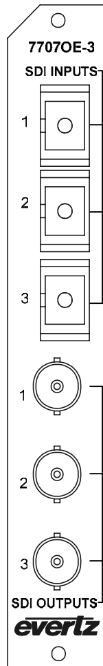
Figure 2-1: 7707OE-3 Rear Panel
