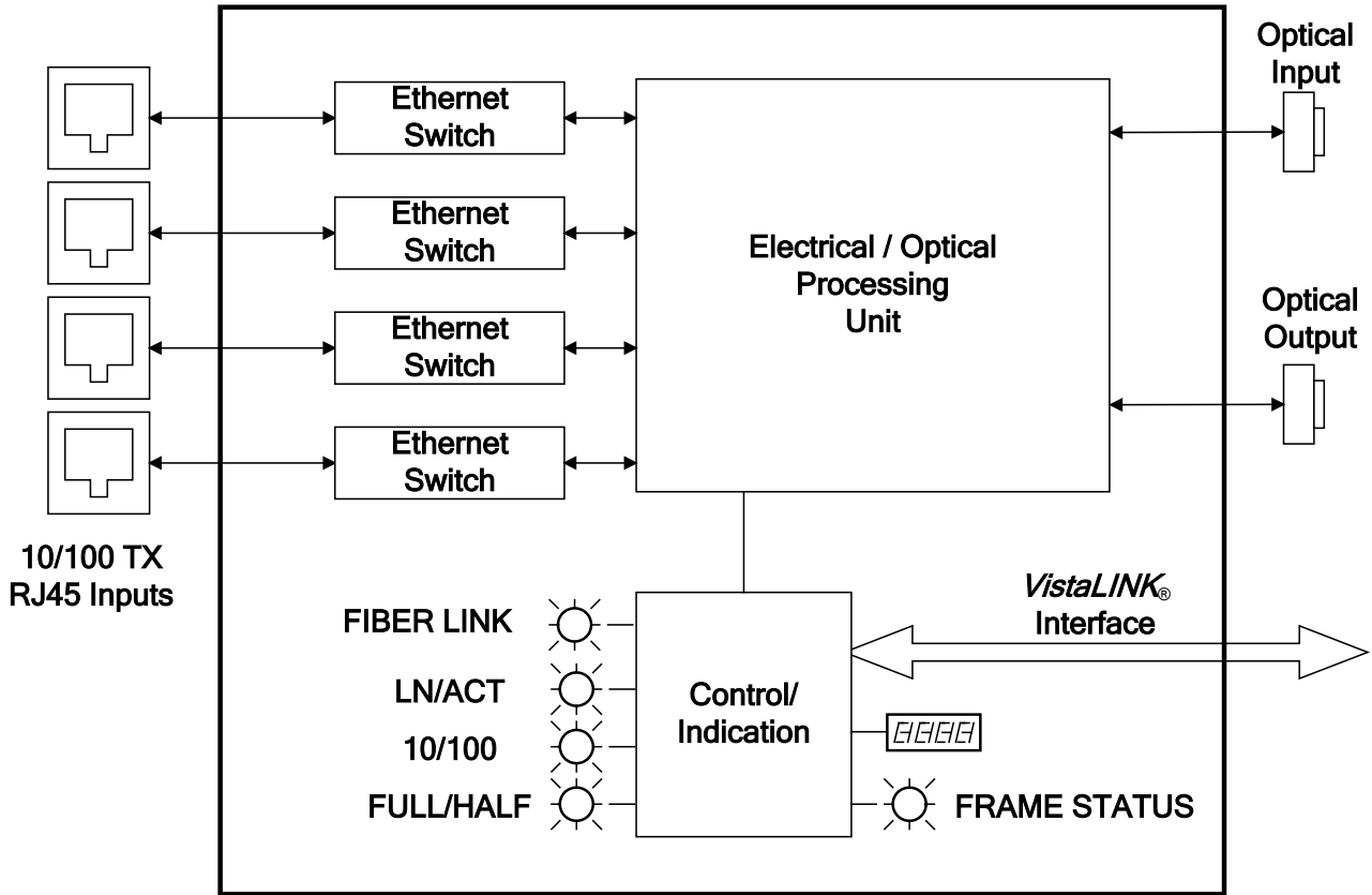
Figure 1-6: 7707ET-4-F2 Block Diagram
