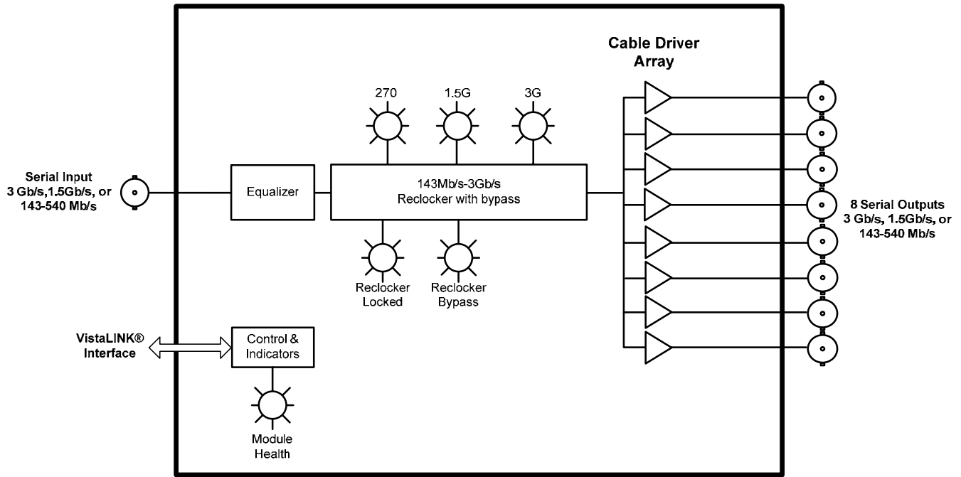
Figure 1-1: 500DA-3G Block Diagram
