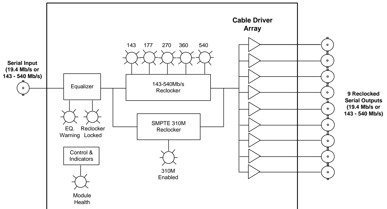
Figure 1-1: 500DA Block Diagram
