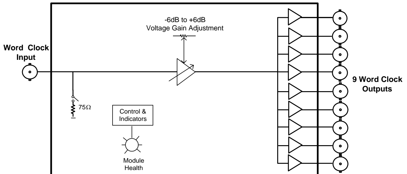
Figure 1-1: 500ADA-W Block Diagram
